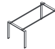
Struttura metallo gamba U US p600/800/900mm Metal structure US U-leg d600/800/900mm Structure en métal pied U US p600/800/900mm
